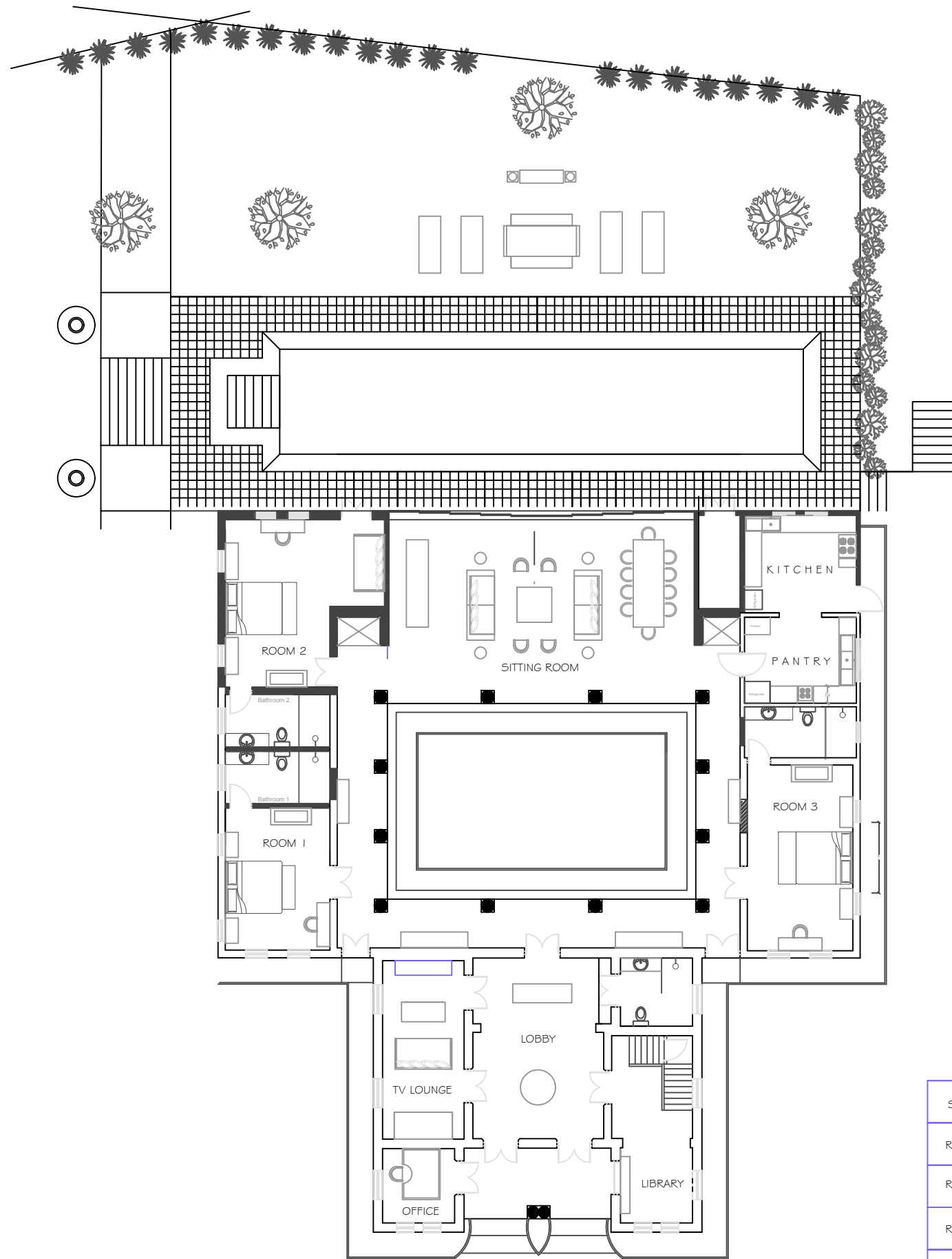
GROUND FLOOR
